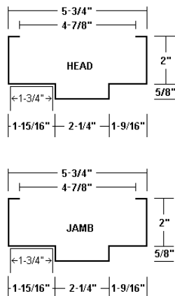
CLIP-IN STEEL STUD ANCHOR
